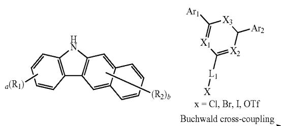
[Reaction Scheme 1]
